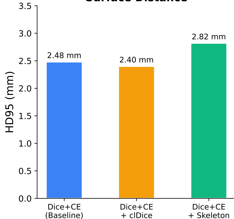
Surface Distance
